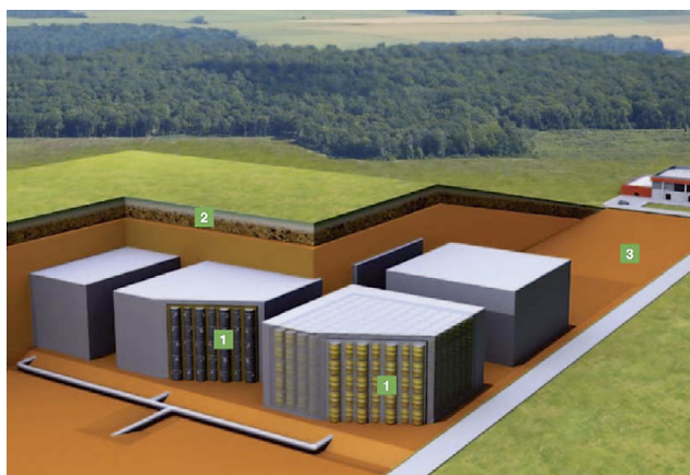
Figure 5: Aube disposal facility disposal concept ( ANDRA, 2011 ) (1) waste package, (2) the final cap, (3) the geological environment of the site (clay aquiclude overlain by a sand aquifer)
