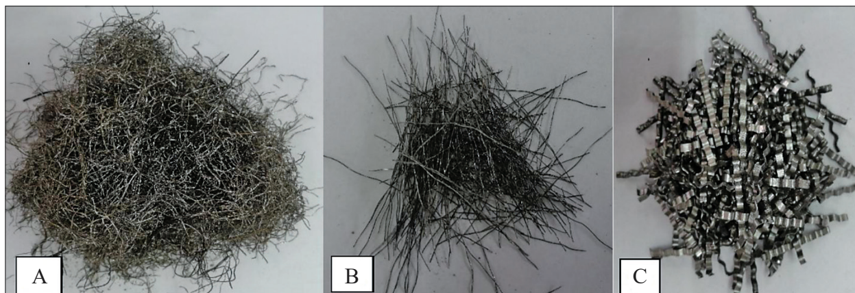
Figure 2: The steel fibres used are (A)- mixed recycled fibres (type 2), (B)- coarse recycled fibres (type 1), and (C)- corrugated industrial fibres.
