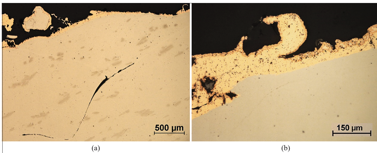
Figure 3: Cross-sectional view of the steel plate material to the surface of the formed through-hole:
