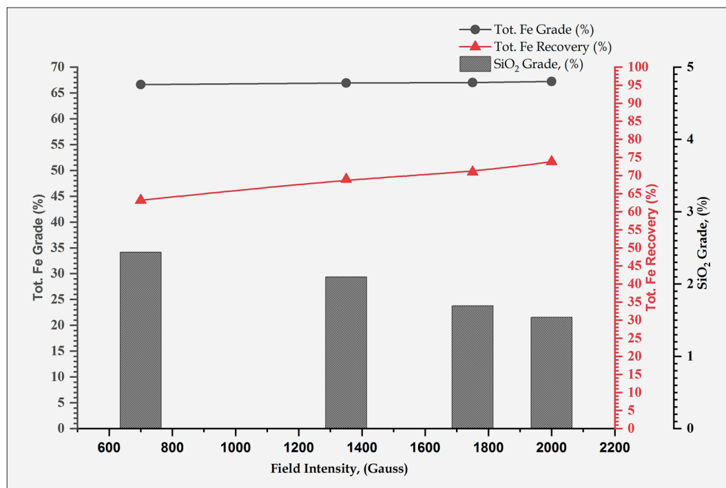
Figure 11: Effect of magnetic field intensity on the reduced Um Nar BIF
