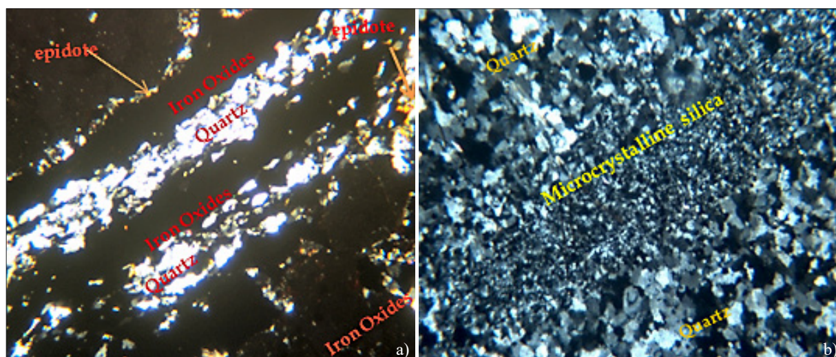
Figure 6: Photomicrographs of thin section (a) showing the alternating bands of segregation composed of quartz (white) and other silicate minerals alternating with iron oxides (black) and other mafic mineral (b) revealing the presence of microcrystalline silica (25X, C.N).
