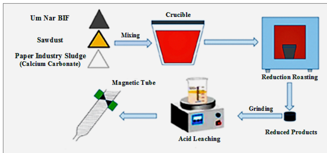
Figure 3: Graphical abstract for the experimental work
