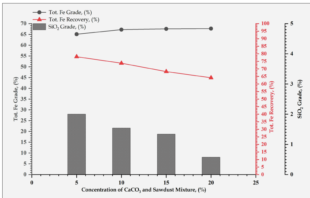
Figure 8: Effect of CaCO 3 and sawdust mixture concentration on tot. iron grade, tot. iron recovery and silica content
