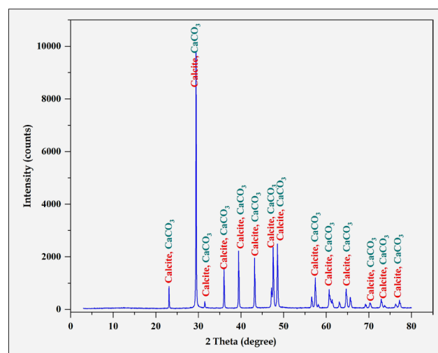
Figure 7: X-Ray diffraction analysis of the paper industry sludge
