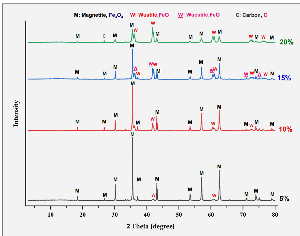
Figure 9: XRD patterns of reduced Um Nar BIF under different dosages of reductant
