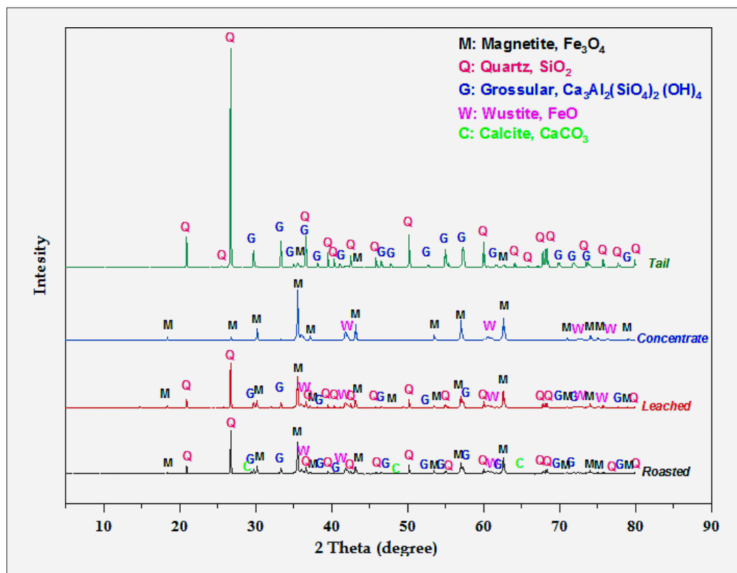
Figure 10: XRD patterns of roasted ore, leached ore, iron concentrate and tail in the presence of 10% dosage of reductant
