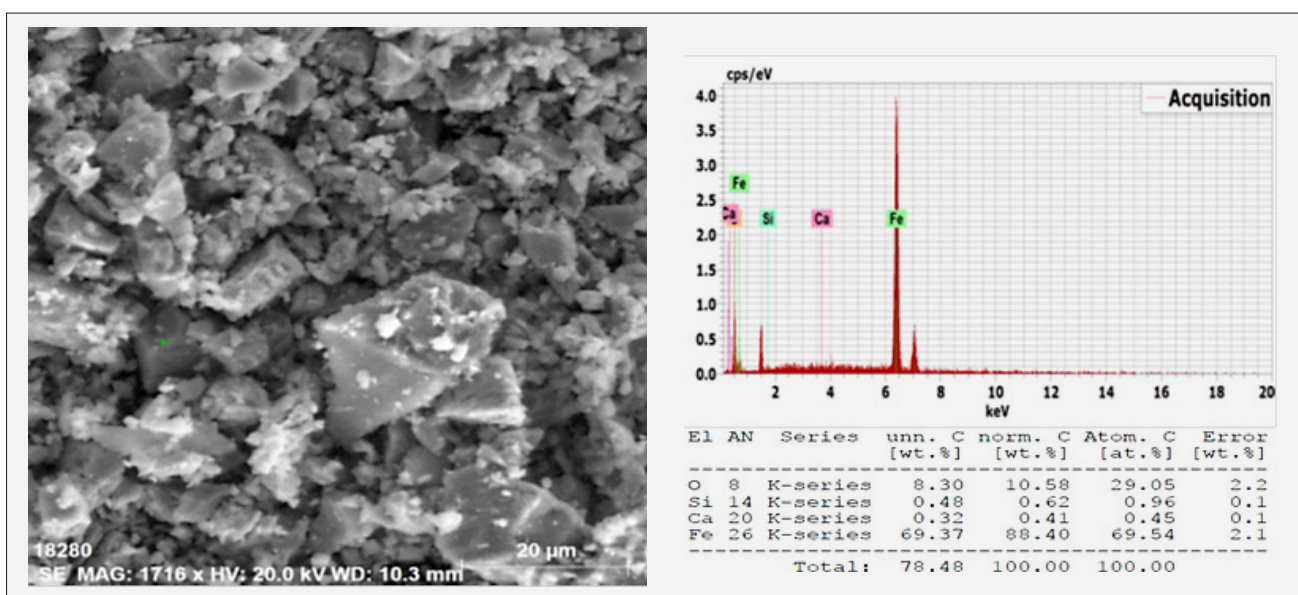
Figure 13: SEM-EDS results of reduced and separated Um Nar BIF with a 10% dosage of mixture of CaCO 3 and sawdust
