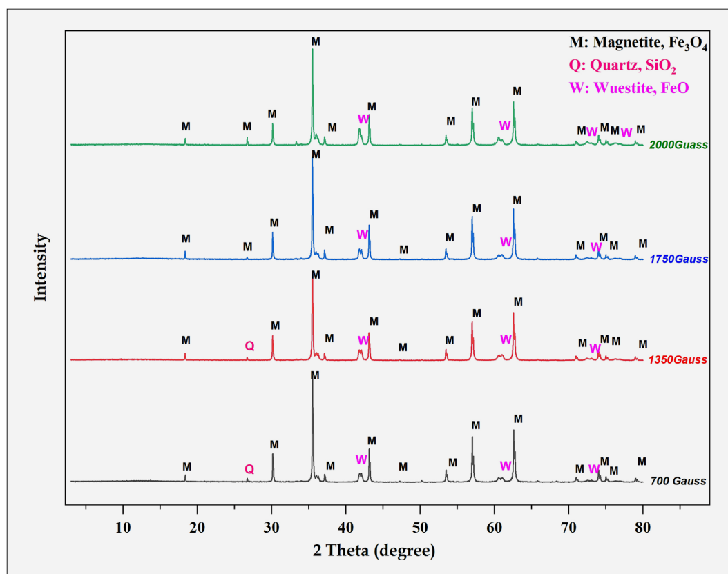
Figure 12: XRD patterns of reduced Um Nar BIF at different magnetic field intensity in the presence of 10% dosage of reductant
