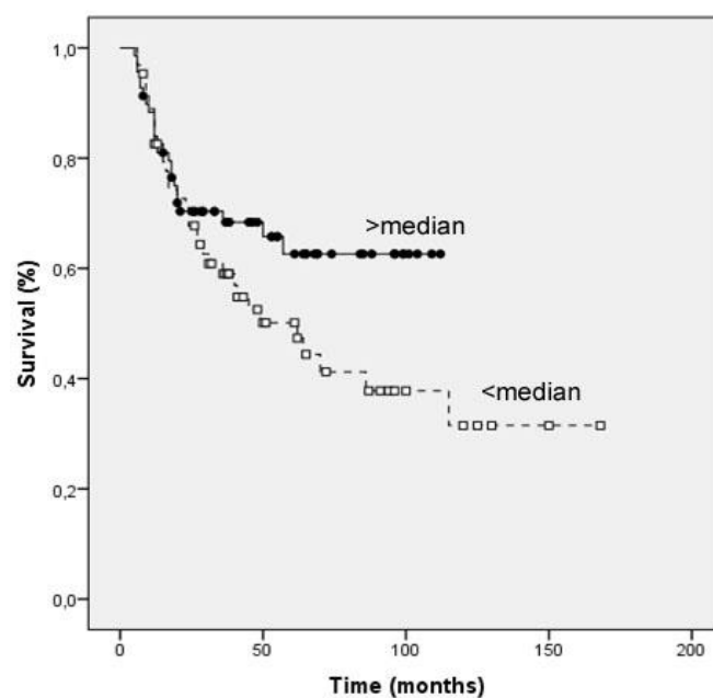
Figure 3. Kaplan-Meier curves of disease-specific survival in the entire study population (N = 133); 2-year survival for NY > median group (n = 69) was 70.3%, and for NY < median group (n = 64) 67.7% ( p = 0.103 log-rank test, p = 0.334 Breslow test, p = 0.206 Tarone-Ware test)
