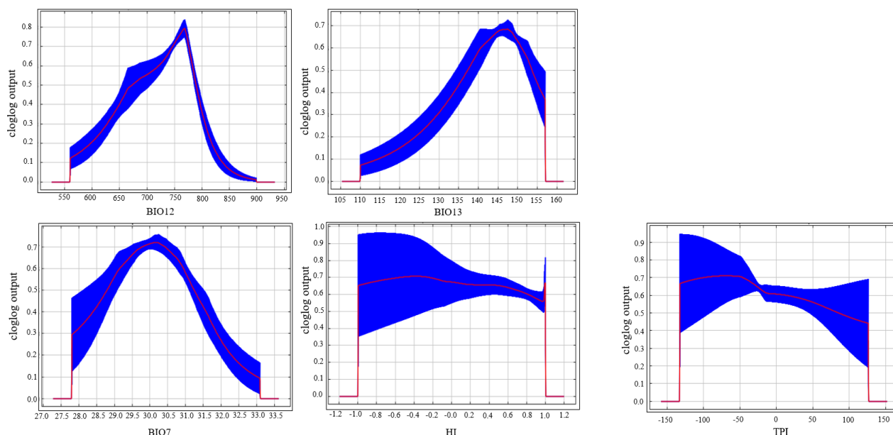
Figure 4. Marginal response curves of model variables of C. monogyna
