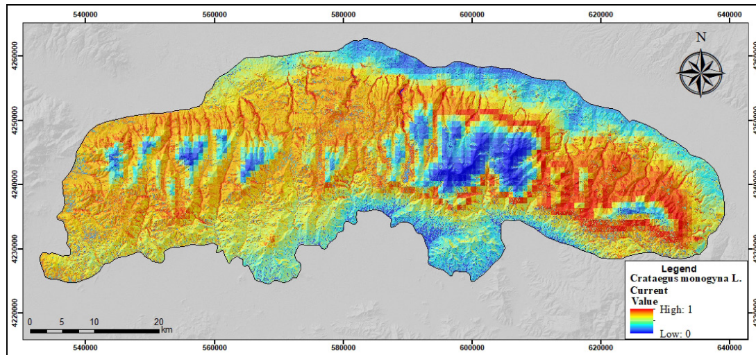
Figure 5. Potential distribution map of C. monogyna using MaxEnt method according to current climatic conditions
