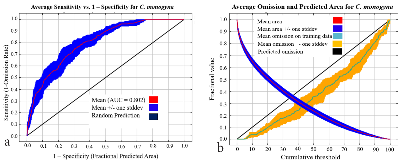
Figure 2. (a) ROC curve and AUC value of C. monogyna ; (b) Plot of mean deficiency and estimated area of C. monogyna Duncan's test results for the number of roots in greenhouse media and phytohormones
