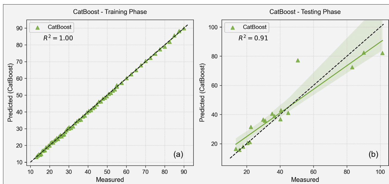
Figure 4: Measured vs. predicted rate of penetration (ROP) in training and testing phases for the CatBoost Model
