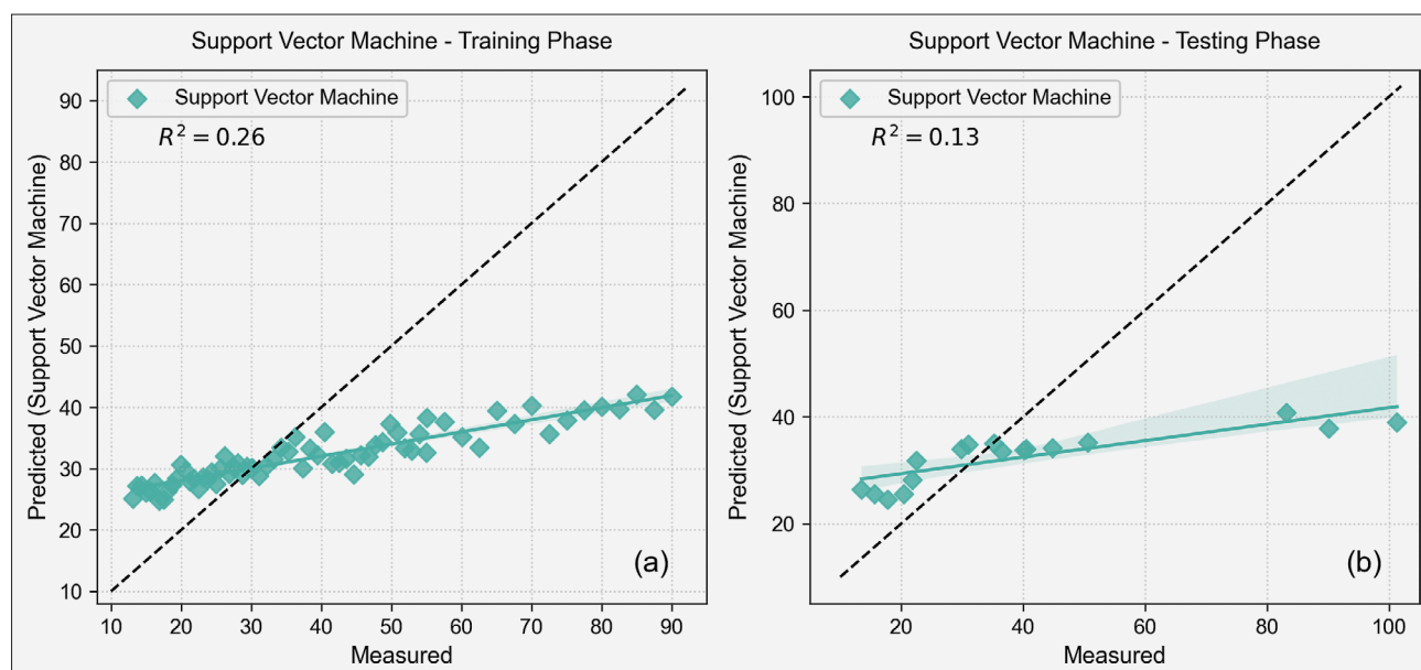
Figure 3: Measured vs. predicted rate of penetration (ROP) in training and testing phases for the SVM Model
