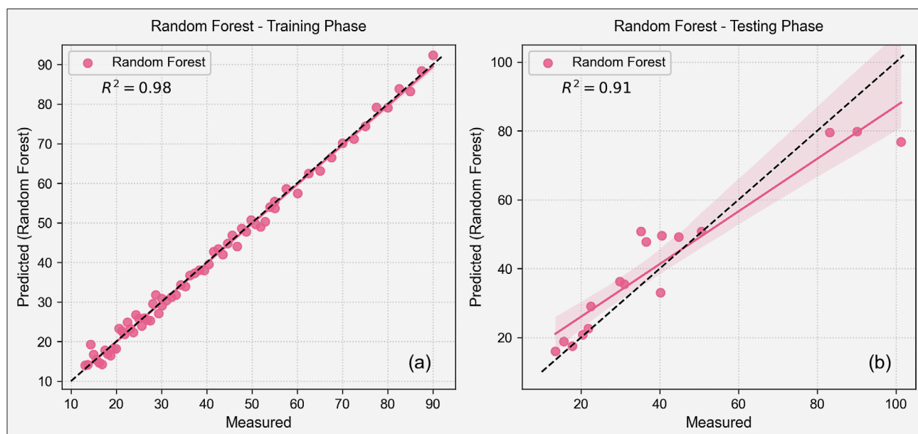
Figure 6: Measured vs. predicted rate of penetration (ROP) in training and testing phases for the Random Forest Model
