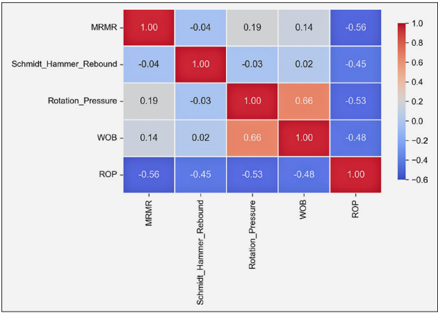
Figure 1: Mapping the correlations between all data samples using a heat map
