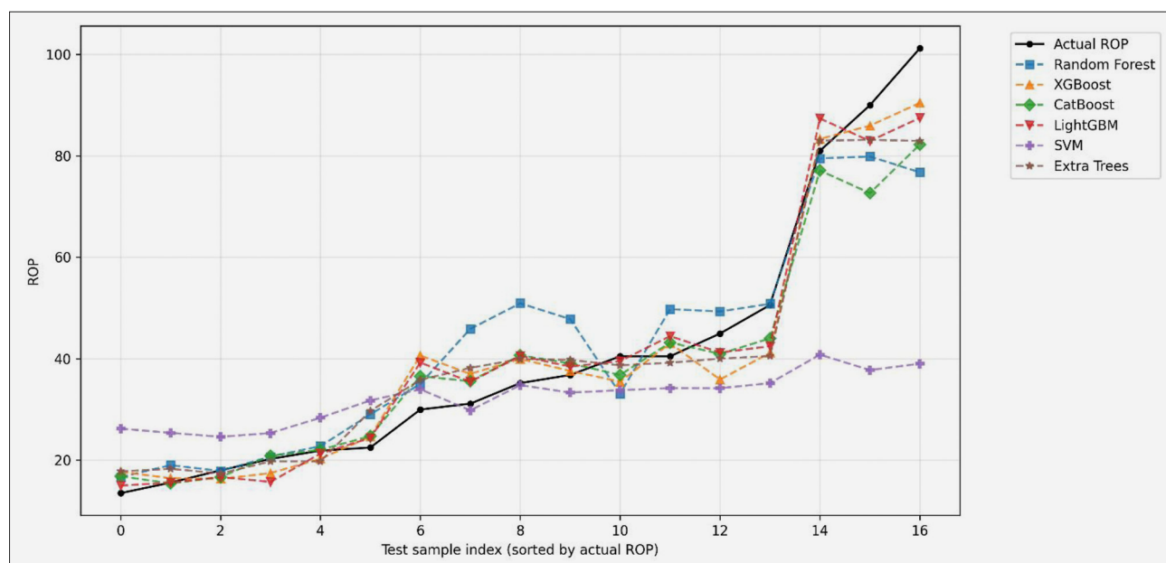
Figure 10: Comparison of predictions by different models with actual data
