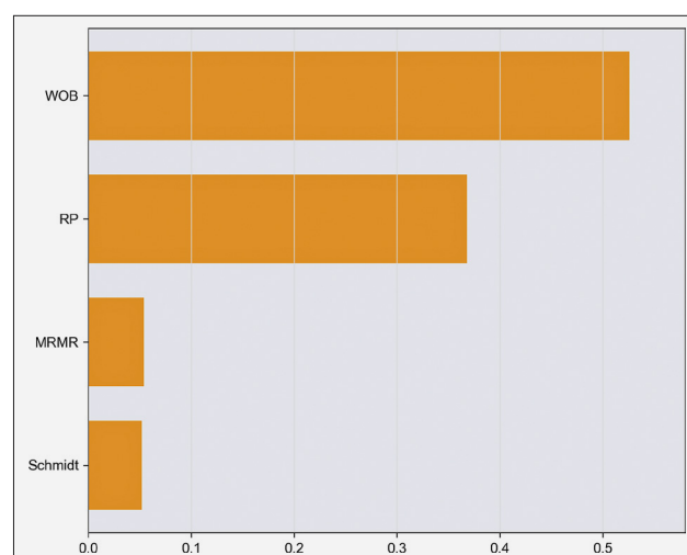
Figure 9: Comparison of influential features in ETR model
