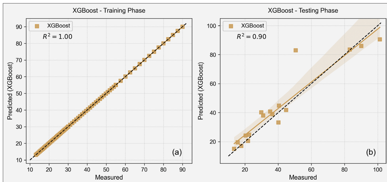
Figure 5: Measured vs. predicted rate of penetration (ROP) in training and testing phases for the XGBoost Model
