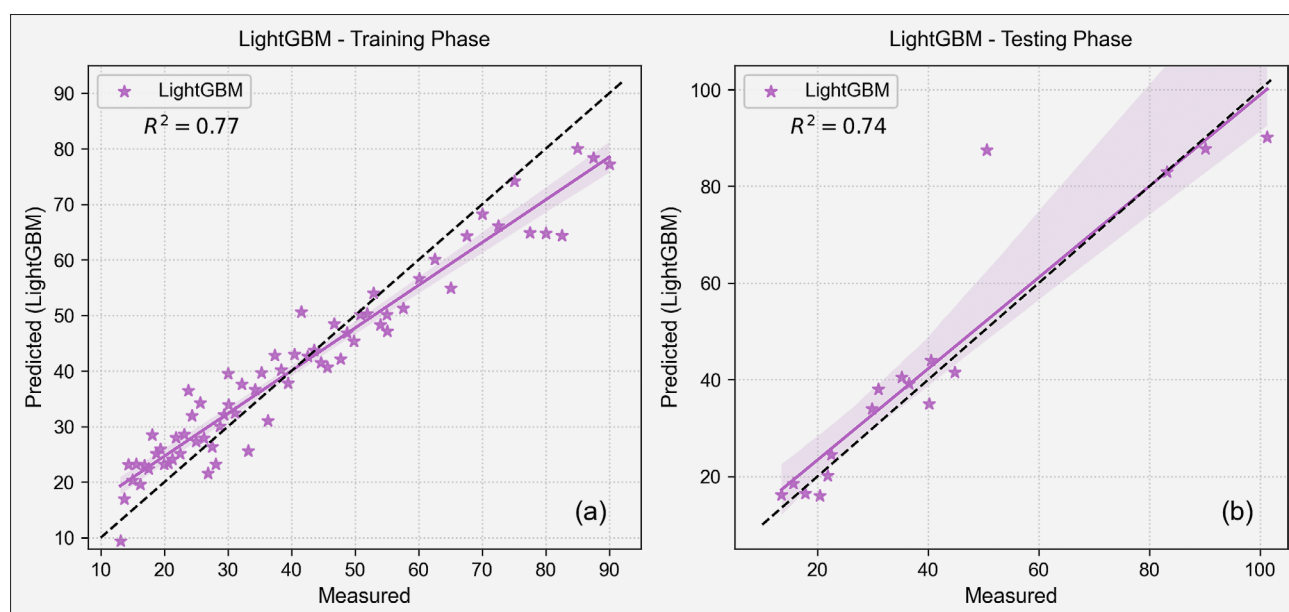
Figure 8: Measured vs. predicted rate of penetration (ROP) in training and testing phases for the LightGBM Model
