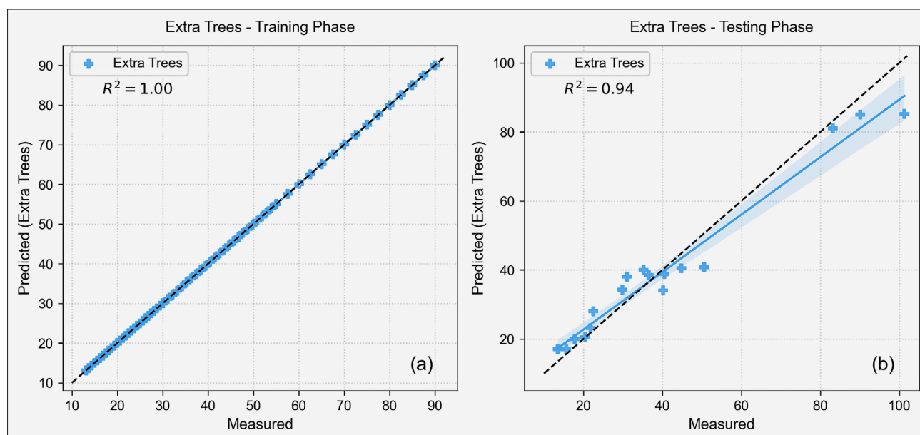
Figure 7: Measured vs. predicted rate of penetration (ROP) in training and testing phases for the Extra Trees Model
